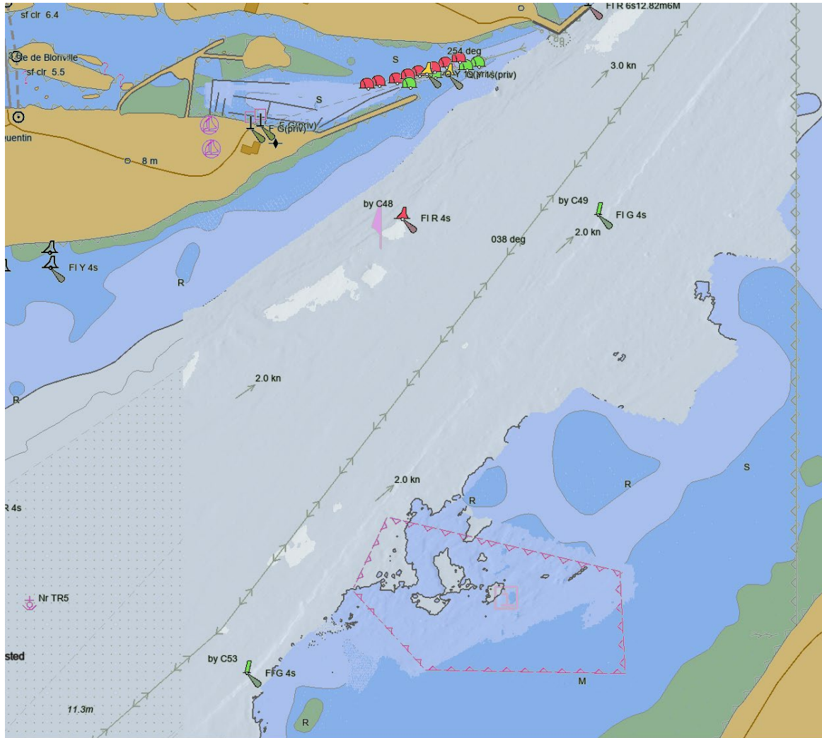
Image 5.3: S-104 chart (courtesy of Primar)
