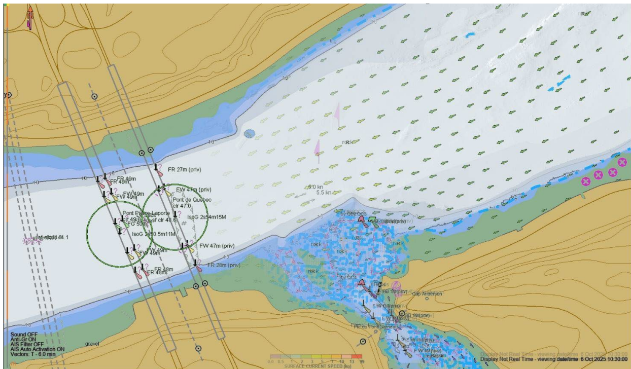
Image 1.1: Example of a merged S-57 and several S-100 Layers taken from the ECDIS Procedures Guide 2026 – 2027 Volume 2
