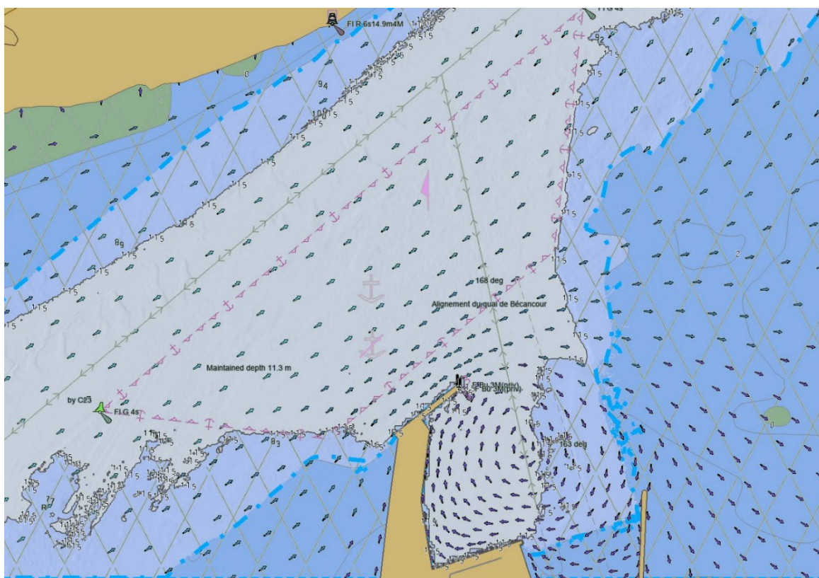
Image 7.1: S-101, S-102, S-104 and S-111 chart (courtesy of Primar)
