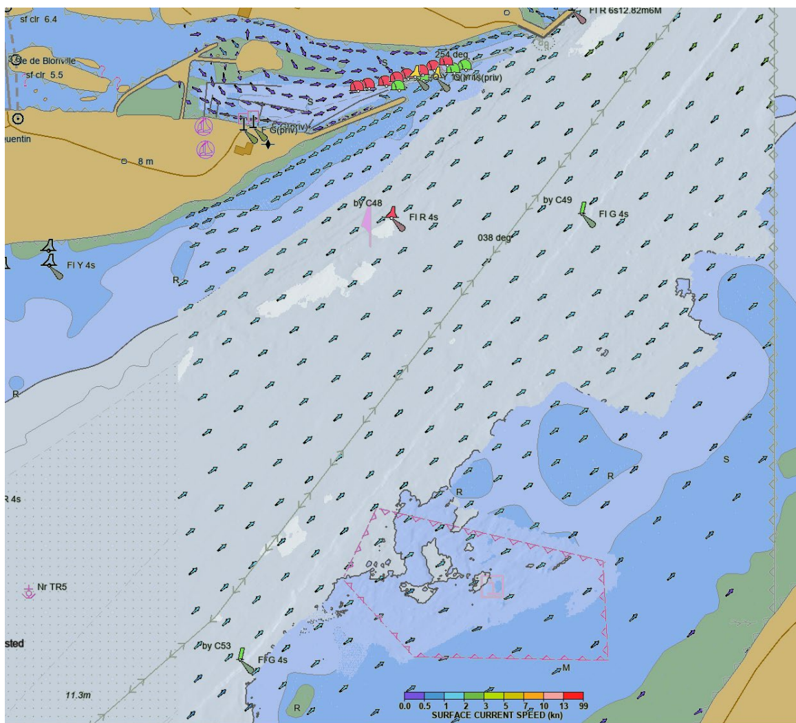
Image 6.1: S-111 chart (courtesy of Primar)
