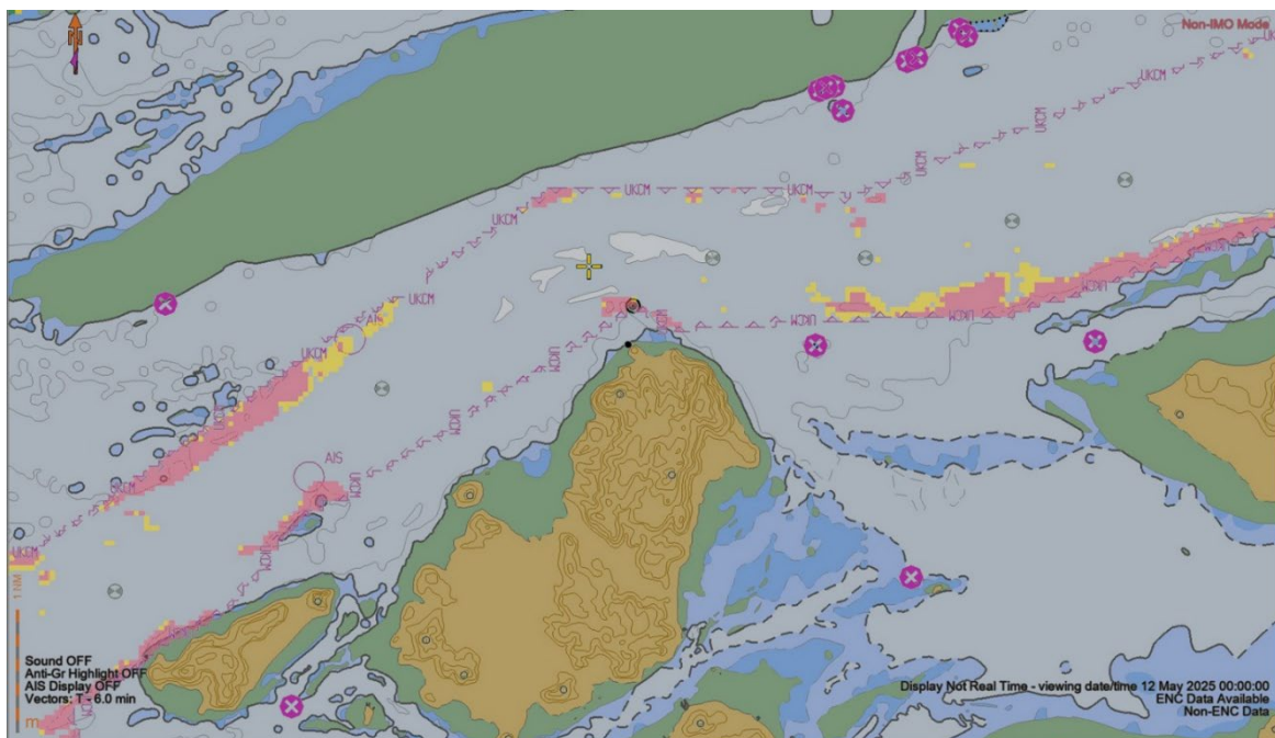
Image 6.4: S-128 chart (courtesy of OSI)
