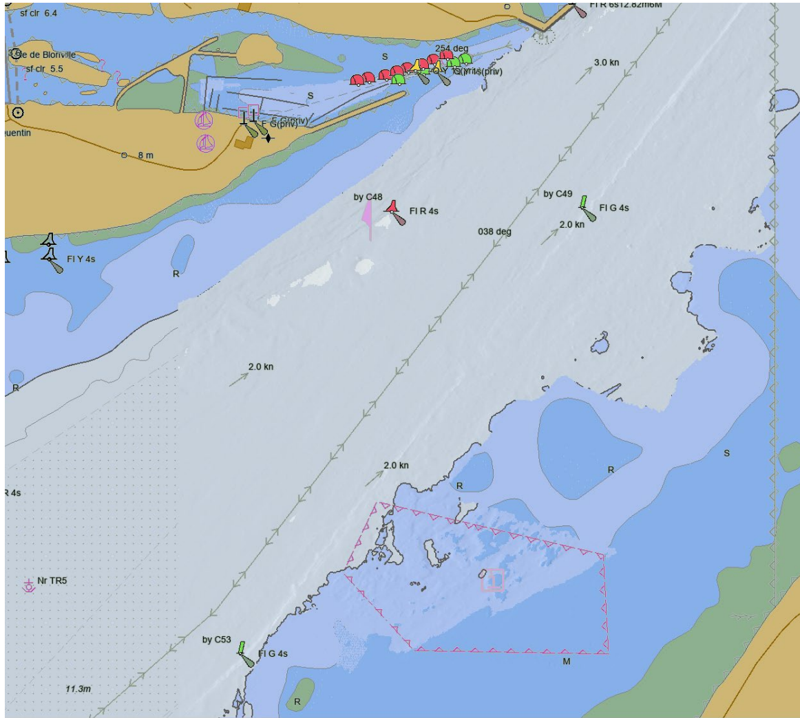
Image 5.2: S-102 chart (courtesy of Primar)
